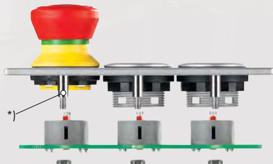
base-plate mounting mounting depth 16.2 mm
