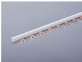
31024 comb type busbar, 1-pole, fork type, pitch 27 mm 80 A, pitch 27 mm, 1 m long 16 mm 2
